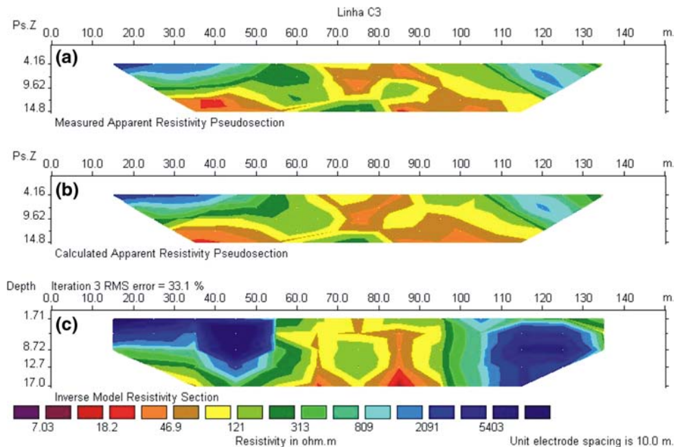
Fig. 3 Resistivity section of the line C3
